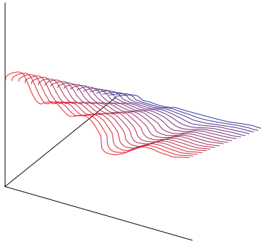
Figure 3. Spectral graph
